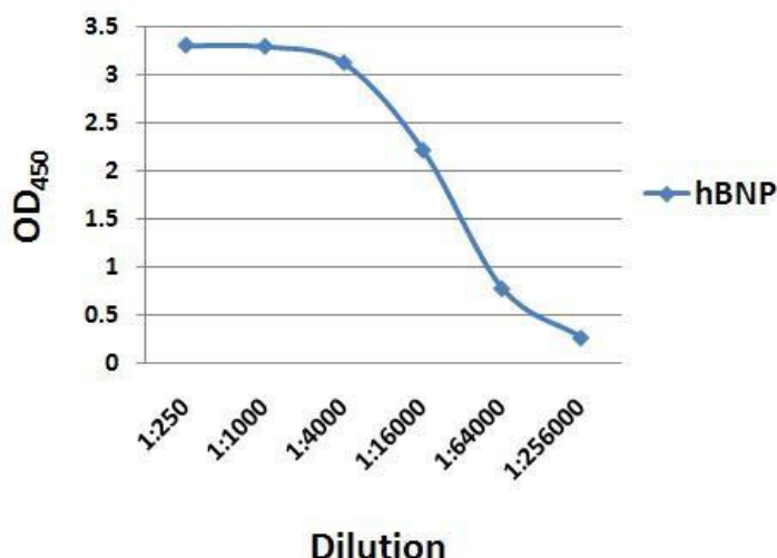
ELISA Profile of IT-010-002
